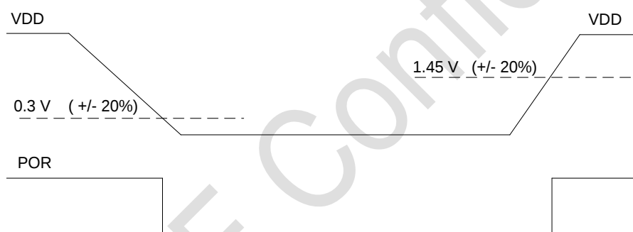
Figure 4. Sudden Decrease of VDD lead to POR Reset
