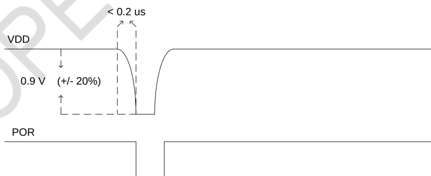
Figure 5. Rapid Decrease in Supply Voltage causes POR Reset
