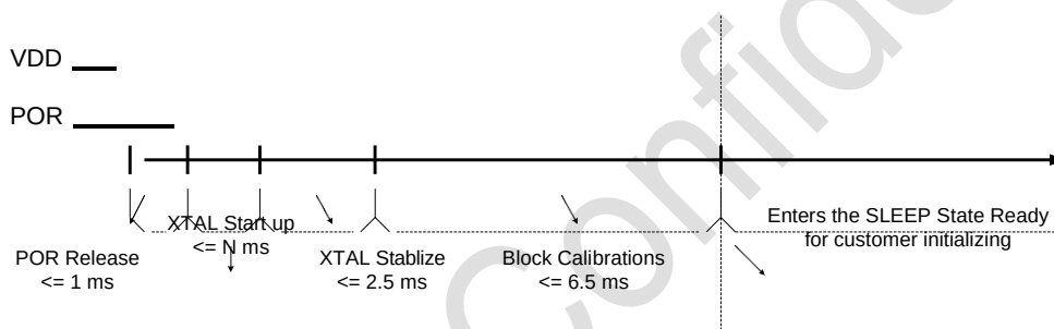
Figure 8. Power on sequence
