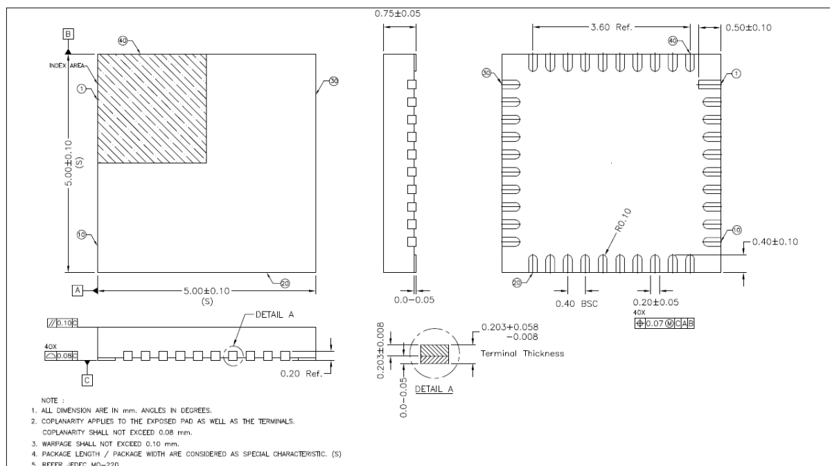
Figure 38: Package Dimensions QFN
