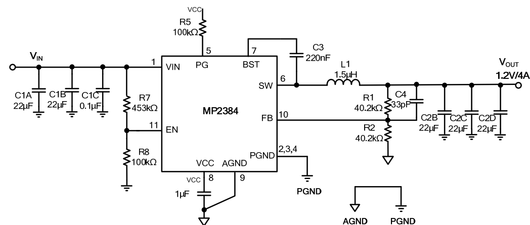
Figure 16: V_{IN} = 19V , V_{OUT} = 1.2V/4A
