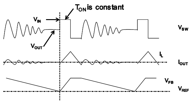
Figure 3: Light-Load Operation
